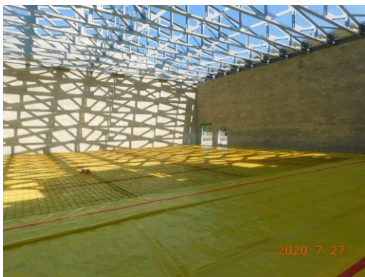
Floor prep taking place for the gym floor concrete pour
