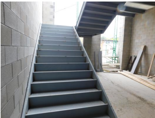
Unit C metal stairs being completed
