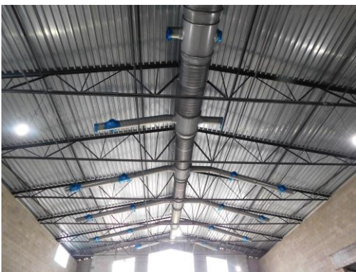
Ductwork continues in the student dining
