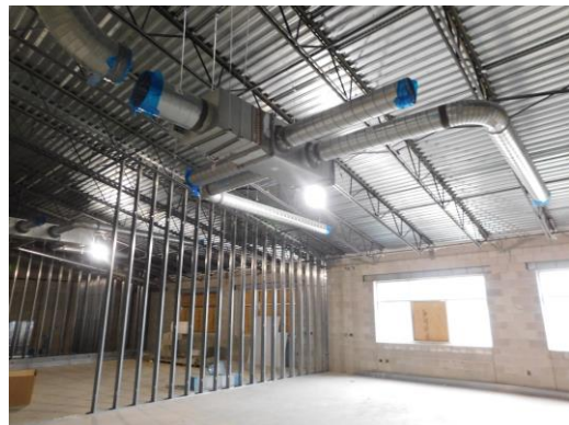
HVAC equipment installation in the classroom wings
