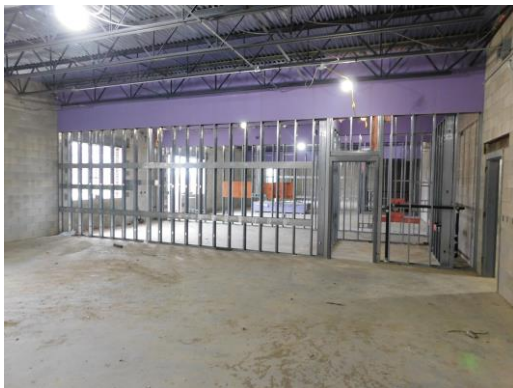
Metal studs and drywall tops installed in the classroom wings
